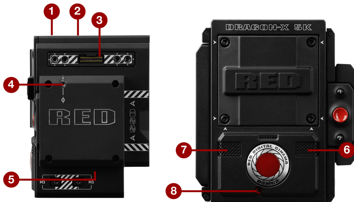
Figure: DSMC2 DRAGON-X Ports and Features
