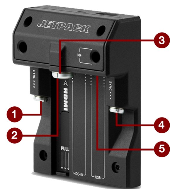
Figure: DSMC2 Jetpack Expander
