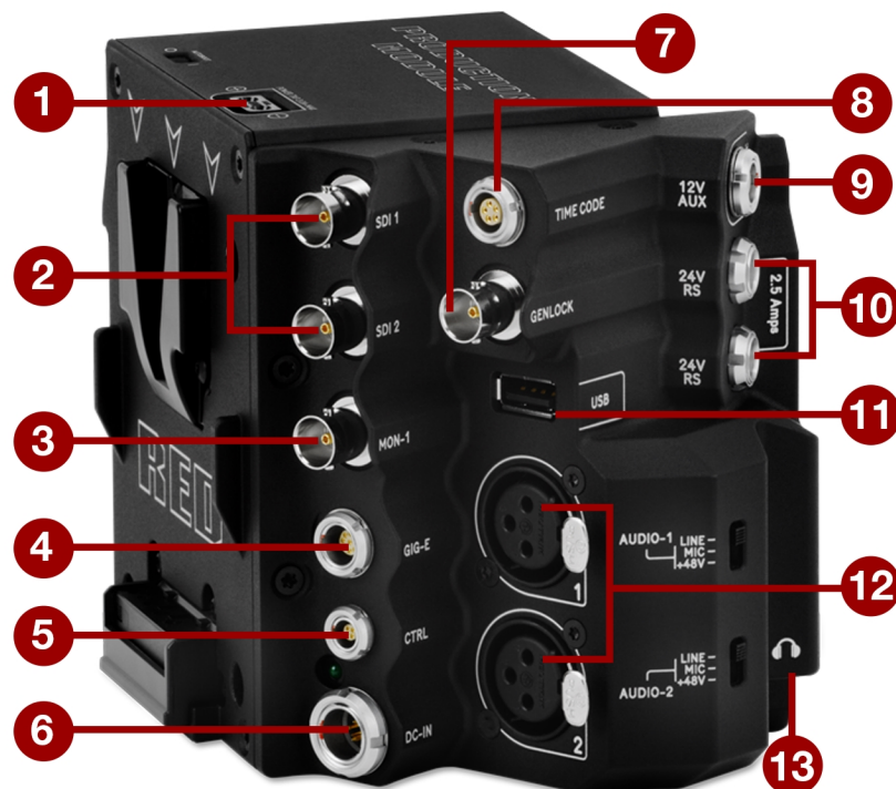
Figure: DSMC2 Production Module (V-Lock Pictured)
