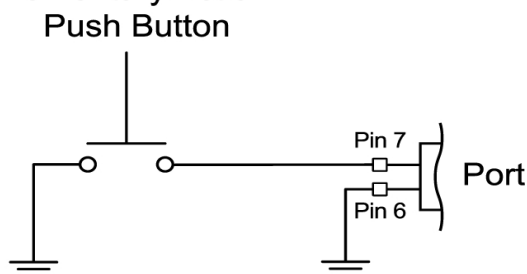
Figure: Contact Closure Style Trigger Button Circuit Diagram
