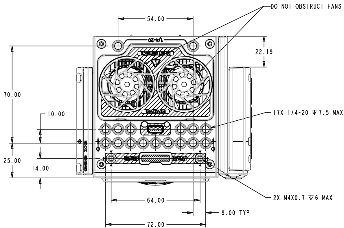
Figure: Camera Top View
