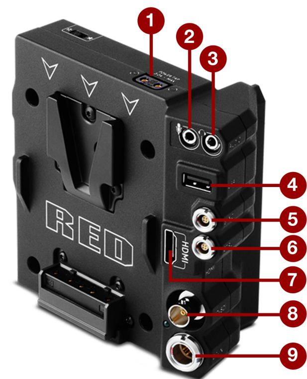
Figure: DSMC2 V-Lock I/O Expander
