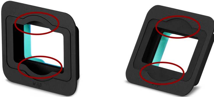
Figure: Original DSMC2 S35 OLPF, Curved Glare Stops (Left); and Modified DSMC2 S35 OLPF, Straight Glare Stops (Right)
