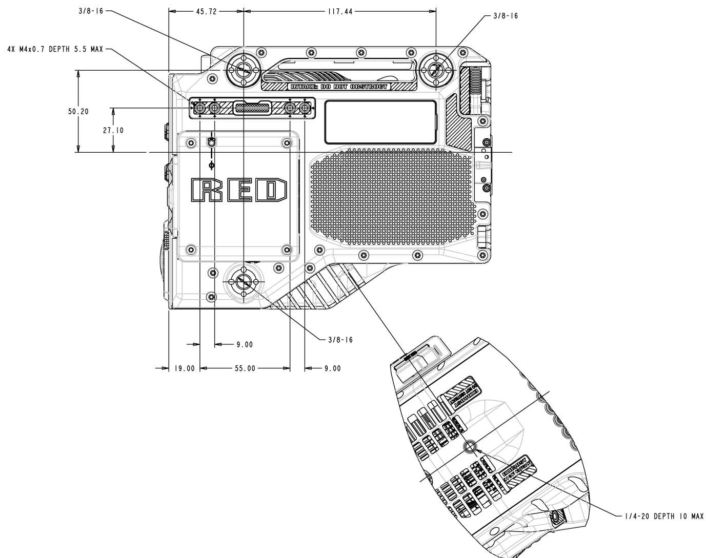
Figure: Camera Side View (Right)
