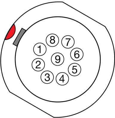
Figure: Front face of the female 9-contact Extension port (looking at the back of the camera). NOTE: The required mating connector is 9-Pin 0L Straight Plug Connector (ODU, part# SX0L0X-P09MCC0-0001).
