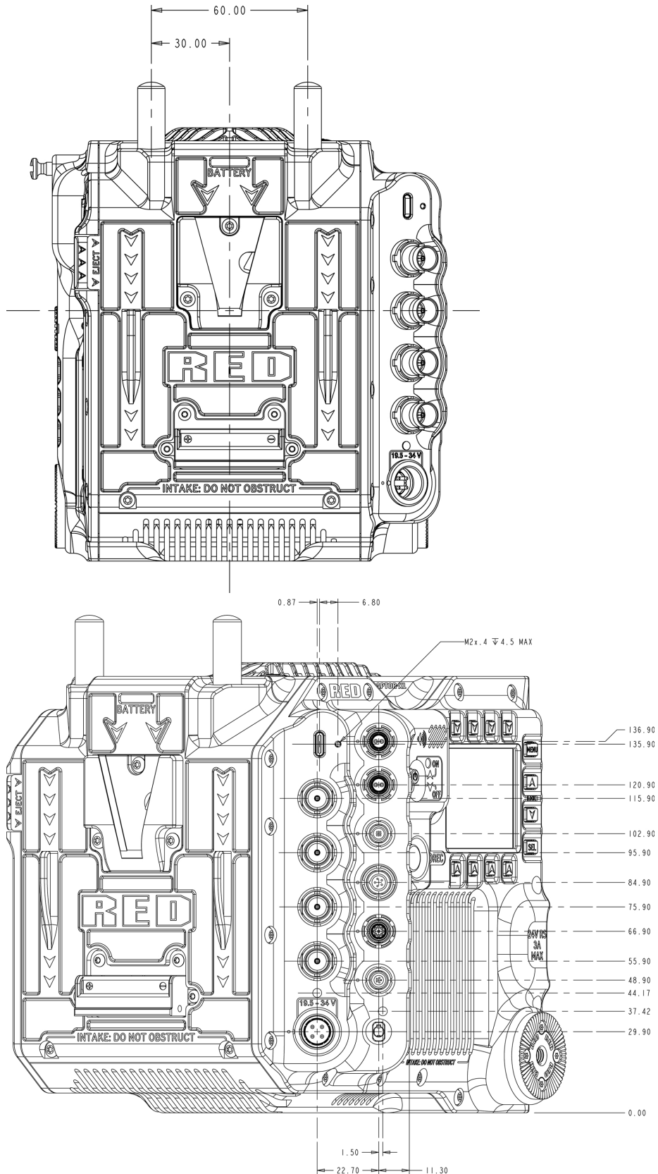
Figure: Camera Back View (V-Lock)
