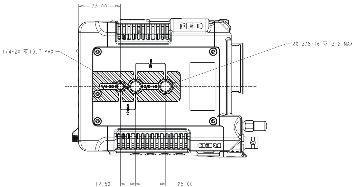
Figure: 摄像机底视图
