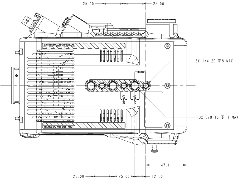
Figure : 摄像机底视图
