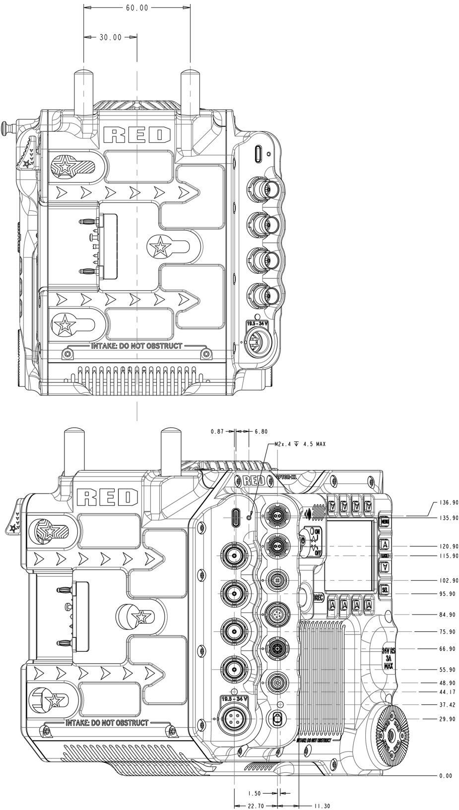
Figure: 摄像机背面图(金装)
